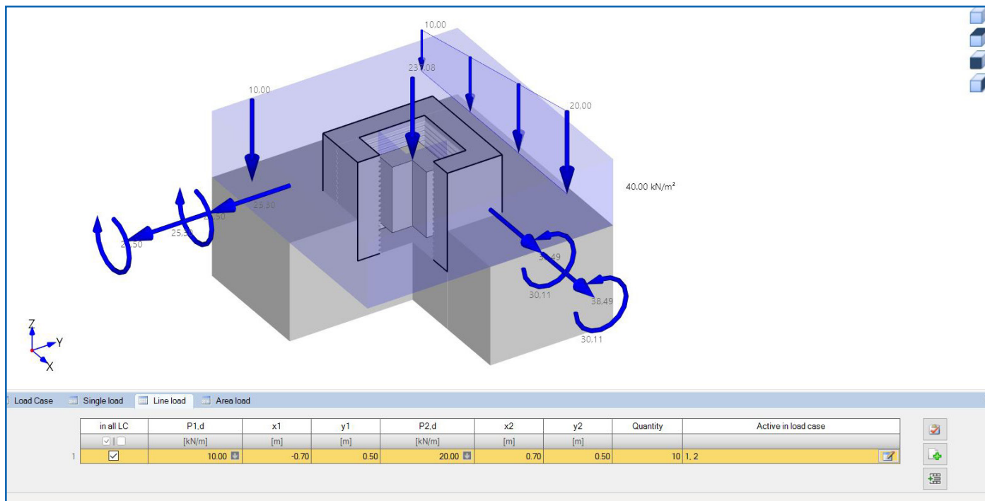
Figure 8: The possibilities of load definition in FRILLO FD+ (column loads and additional loads).
